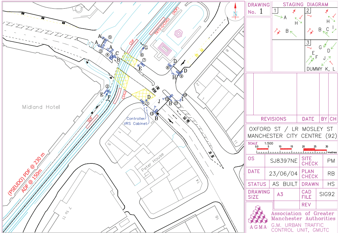
Figure 1 and Figure 2 show the signal arrangement at the project site, the junction at Oxford St/Lower Mosley St (St Peter's Square). The drawings are not to scale.
